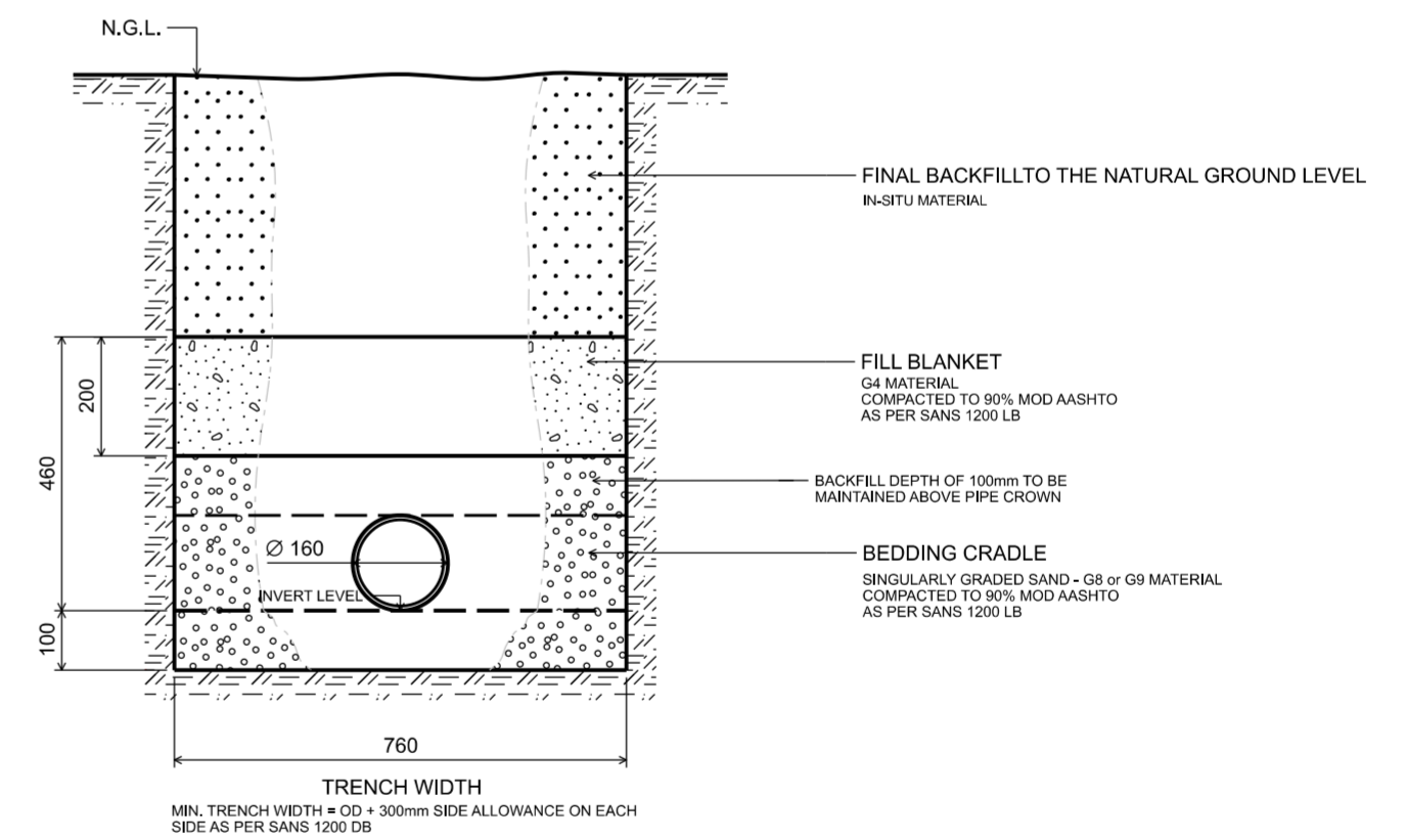
TYPE 4 TRENCH
