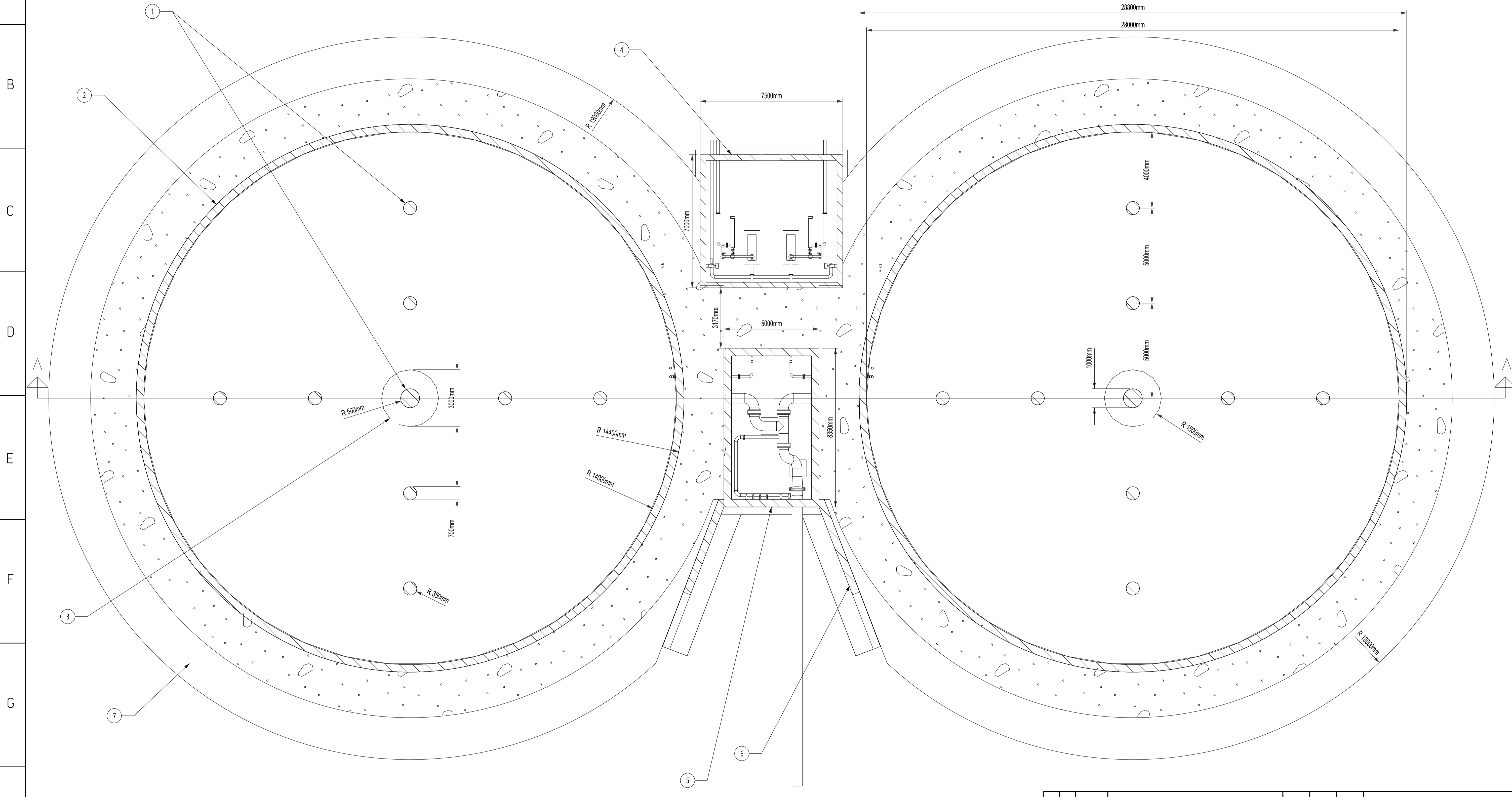
PLAN VIEW
