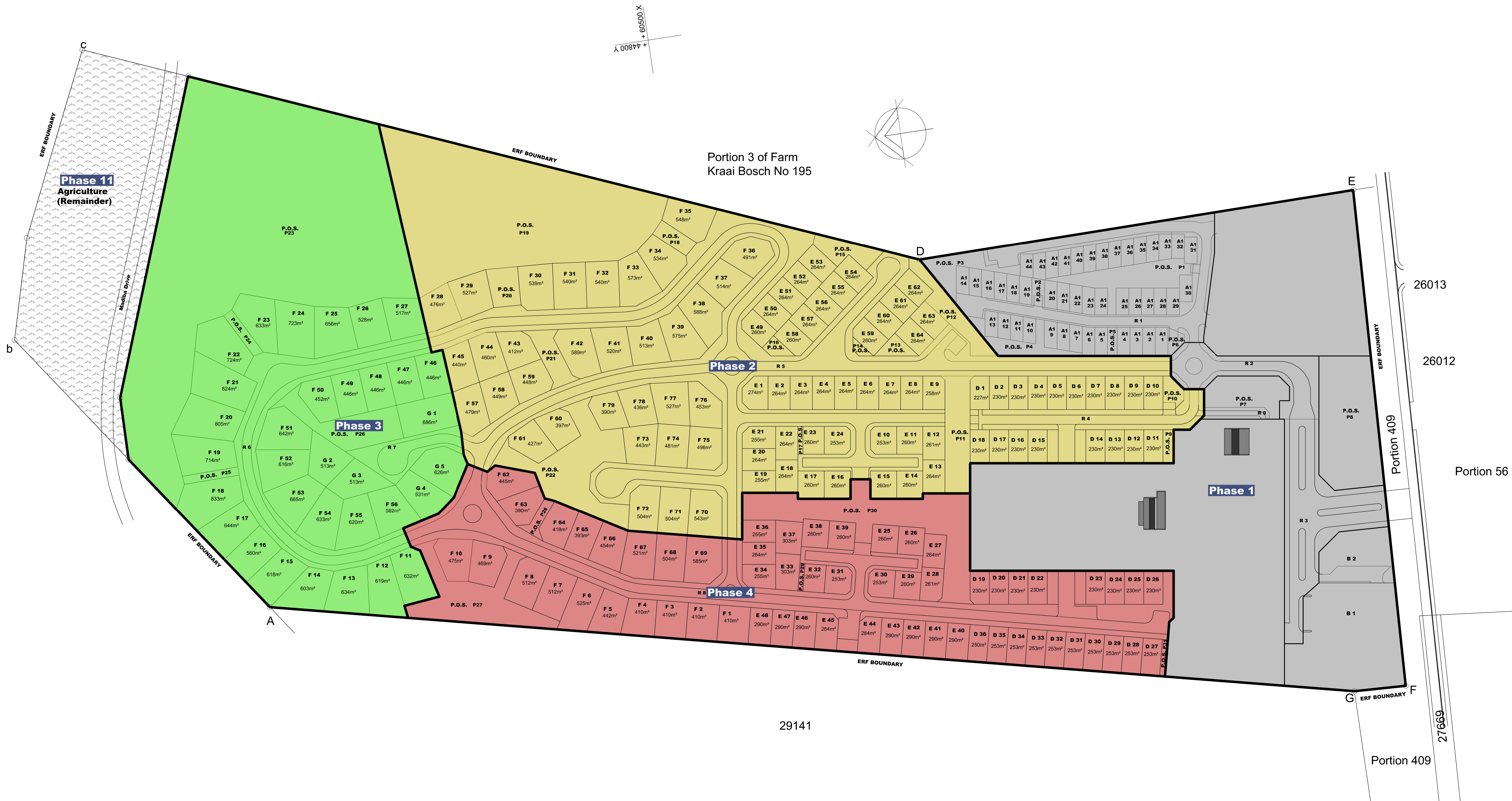
BUILDING & CIVIL WORKS PHASING PLAN scale 1:1250
