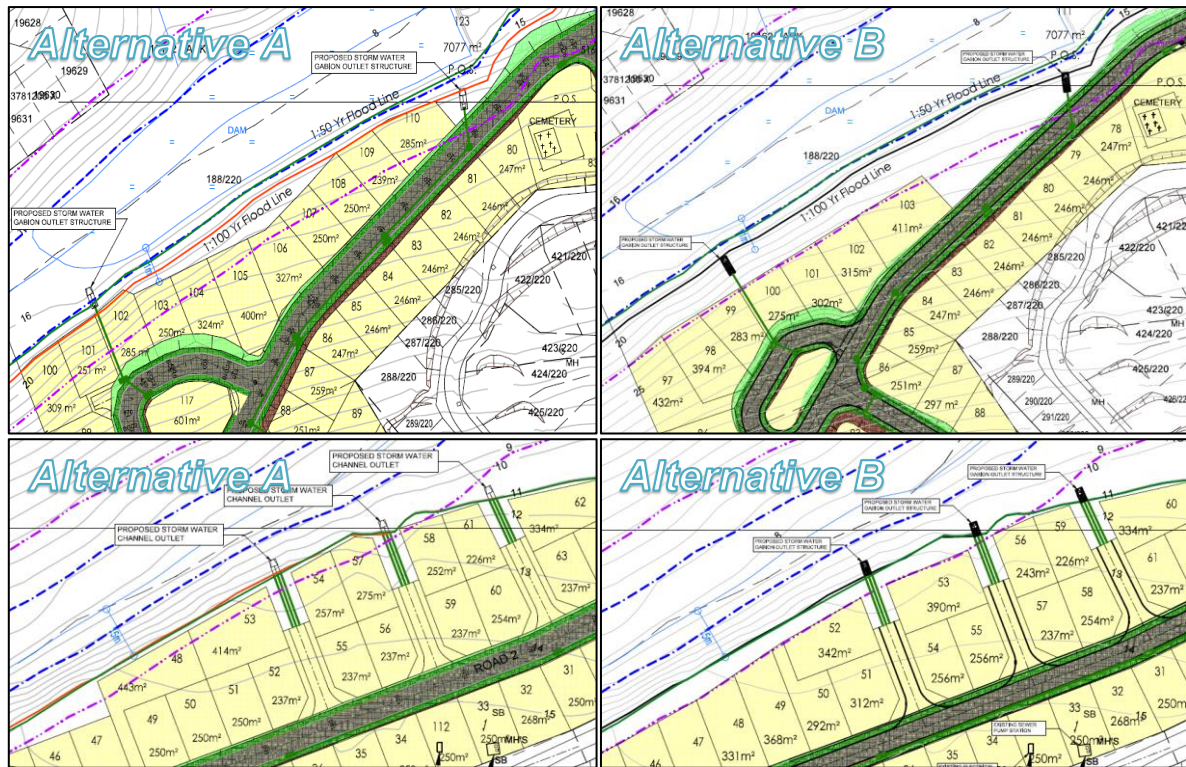
Figure 13: Comparison of Alternative A (left – with erven located in the 15 m buffer – indicated by purple dashed line) and Alternative B (right – erven removed from 15 m buffer – indicated by purple dashed line).
