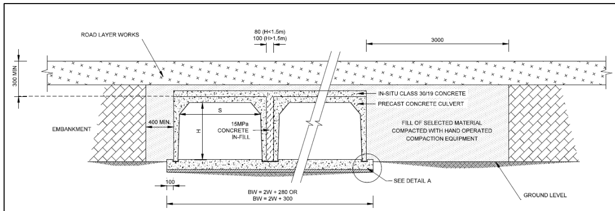
Figure 15: Drawing of proposed concrete culvert bridge
