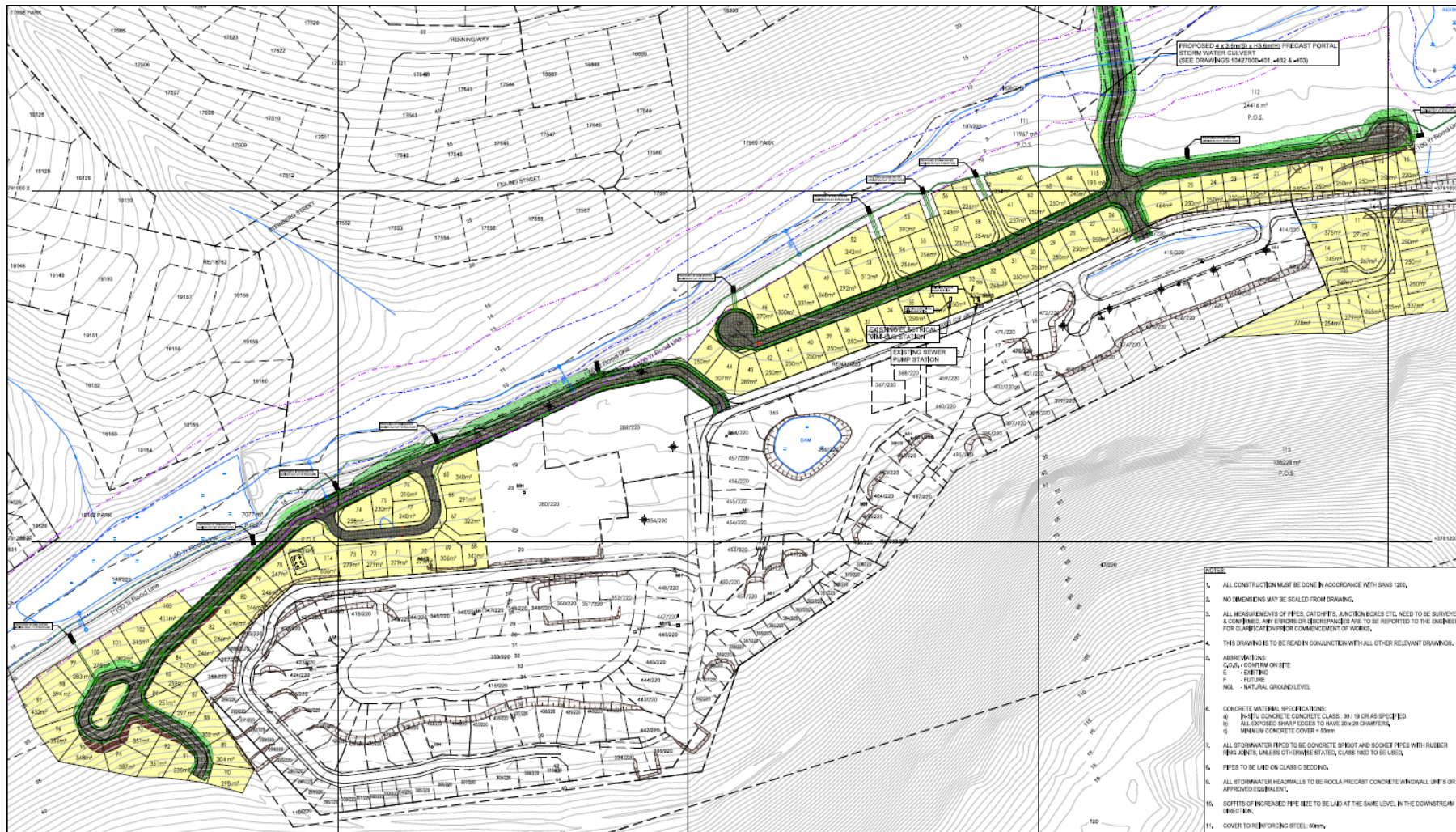
Figure 11: Proposed stormwater layout (Alternative B)
