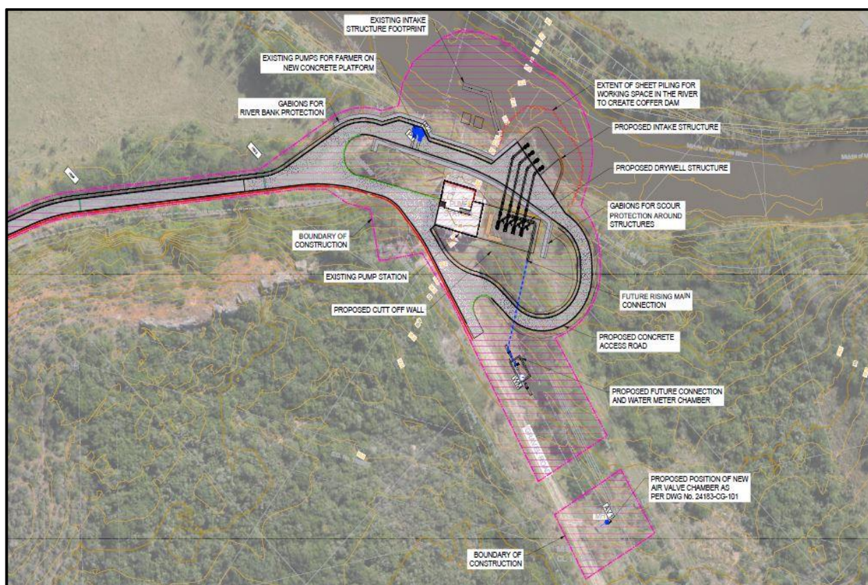
Figure 6: Proposed Upgrades to the Moordkuil Pump Station.
