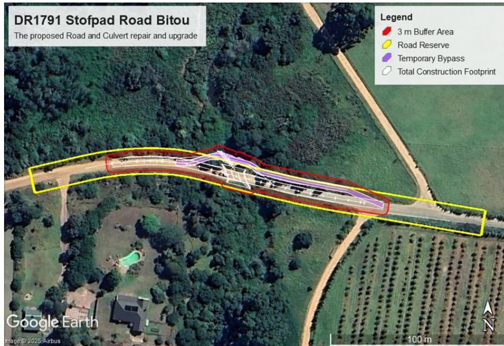
Figure 3. Proposed construction works of the temporary deviation road along DR1791, Wittedrift (downstream).
