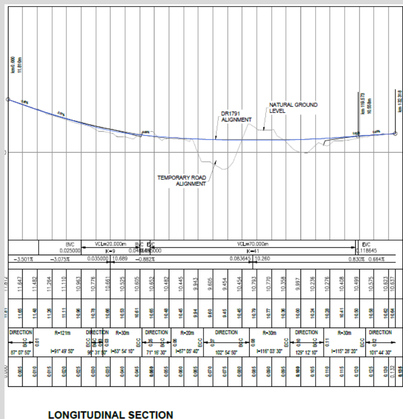
Figure 11. Engineering drawing for the proposed causeway construction located along the DR1791 (Hatch Engineering, 2025).
