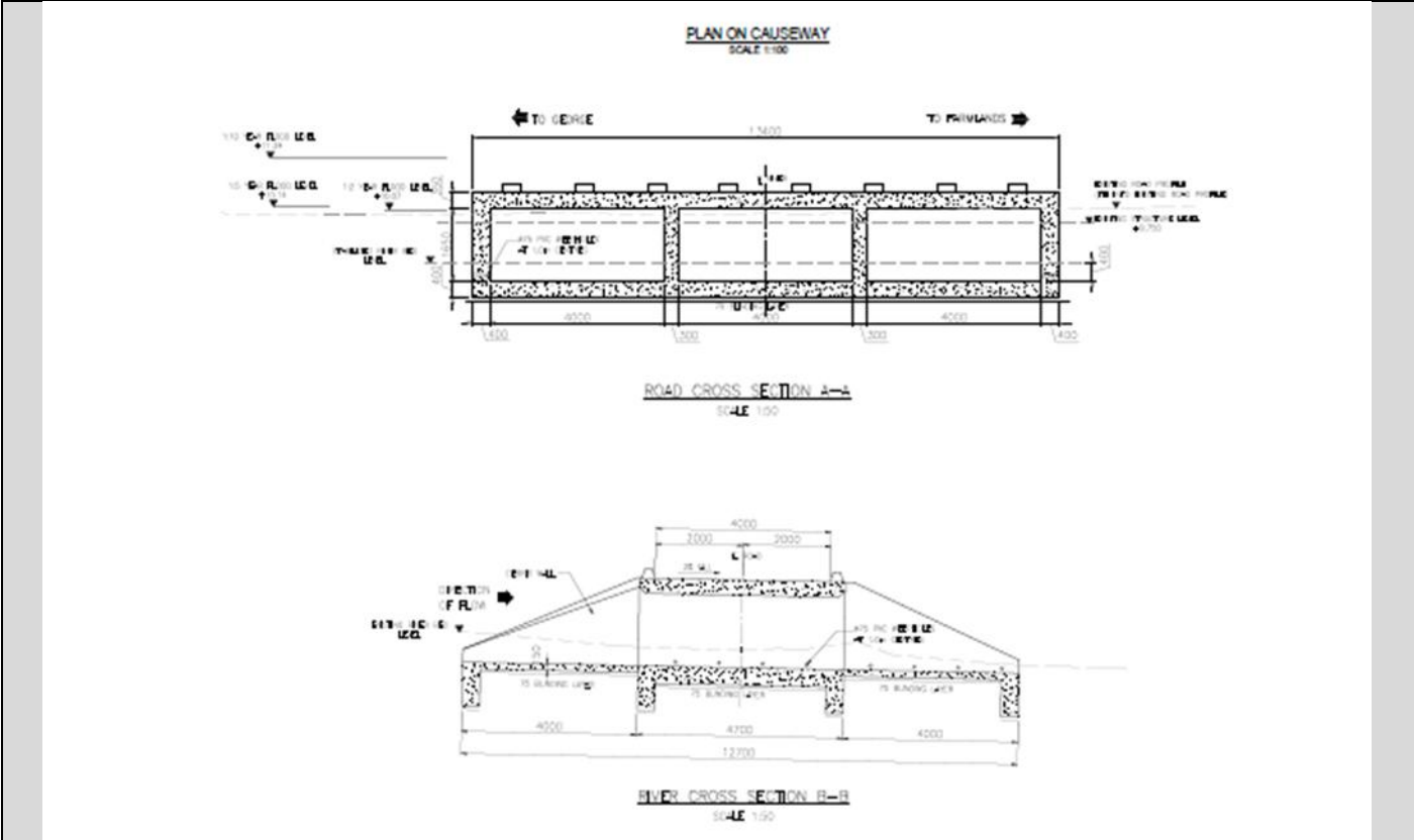
Figure 12. Cross-section of the proposed causeway construction along DR1791, (Hatch Engineering, 2025).
