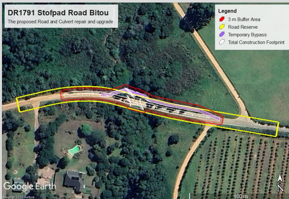
Figure 8. Proposed construction works of the by-pass infrastructure along DR1791, Wittedrift (downstream).
