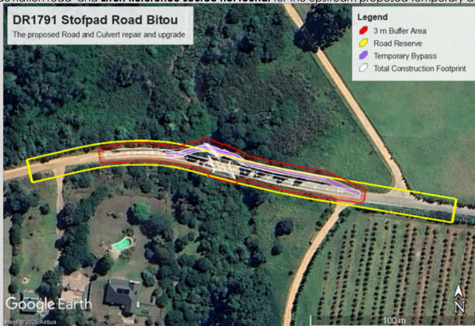
Figure 2. Proposed construction works of the temporary deviation road along DR1791, Witte drif (downstream).
