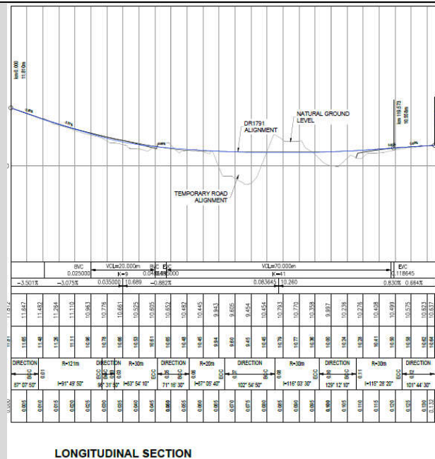
Figure 5. Engineering drawing for the proposed causeway construction located along the DR1791 (Hatch Engineering, 2025).
