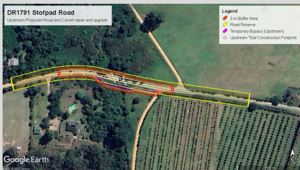
Figure 9. Proposed construction works of the by-pass infrastructure along DR1791, Wittedrift (upstream).
