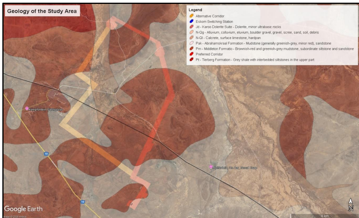
Figure 31: Geology of the study area. The farms are underlain by sedimentary rocks of the Adelaide Subgroup, predominantly dolerite and alluvium.
