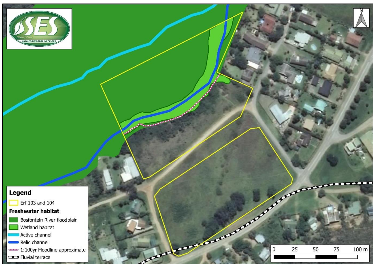
Figure 18: Map indicating the 100-year Recurrence Interval floodline, wetland habitat, as well as the relic and active channel and the floodplain of the Bosfontein River.
