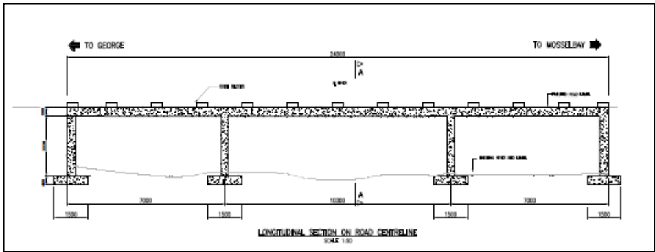
Figure 6. Engineering design of the proposed causeway and associated infrastructure located on DR1602 km 8.4. (Hatch Engineering, 2025).
