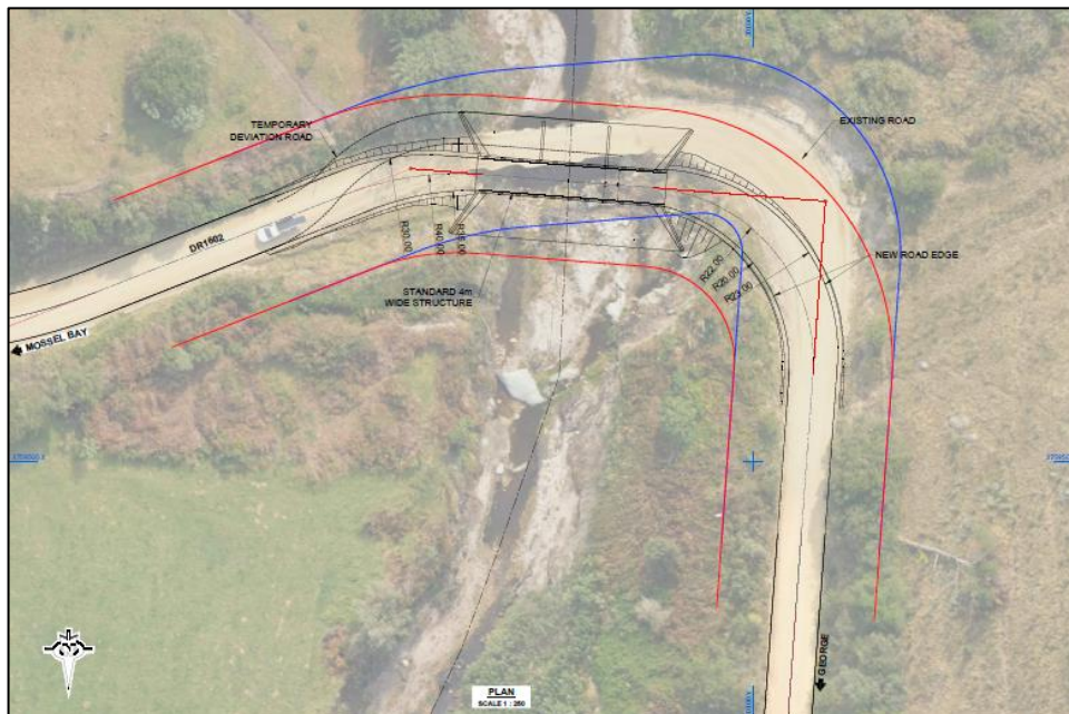
Figure 4. Proposed engineering design of the new proposed causeway and culverts infrastructure located on DR1602 km 8.4. (Hatch Engineering, 2025). Blue lines indicate the current road reserve; red
